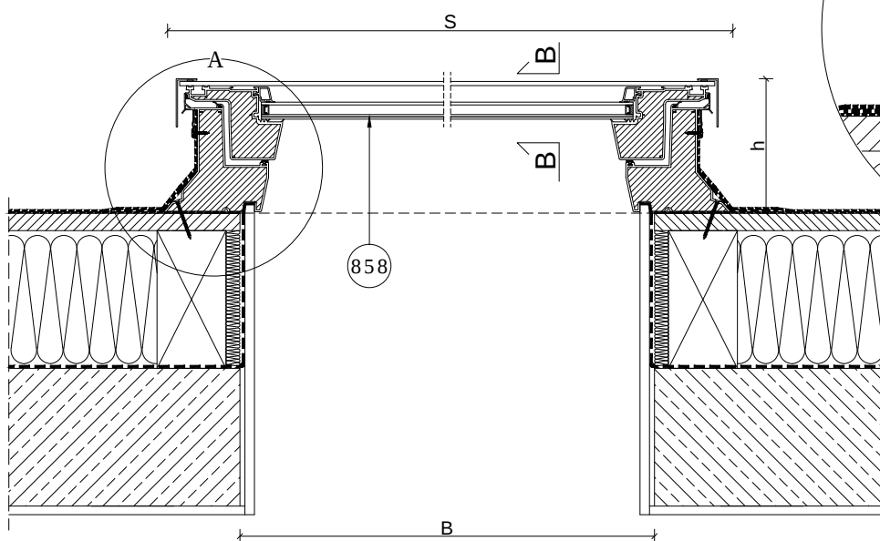
858-DXG P2 Flat Roof Window, non-opened, Flat
